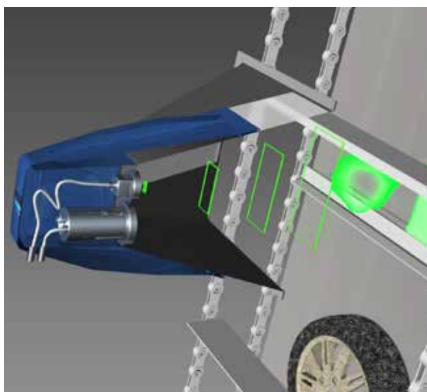
The HUBER Detection System Safety Vision on the RakeMax® screen reliably detects critical matter.
